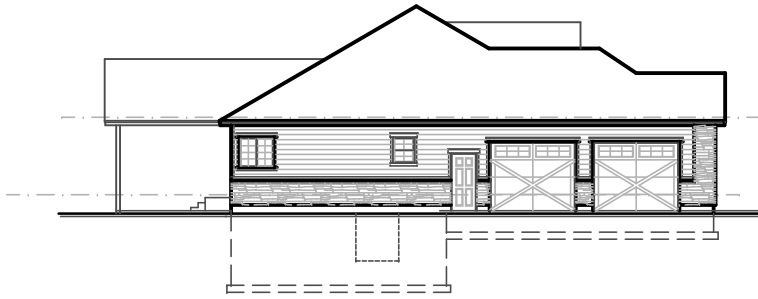
LEFT ELEVATION SCALE 1/8"
