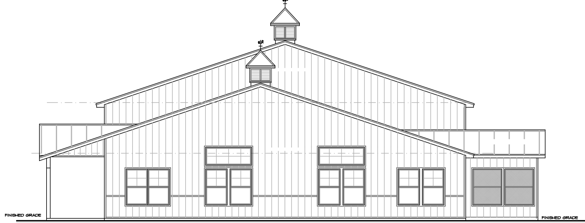
RIGHT ELEVATION SCALE _____ NTS
