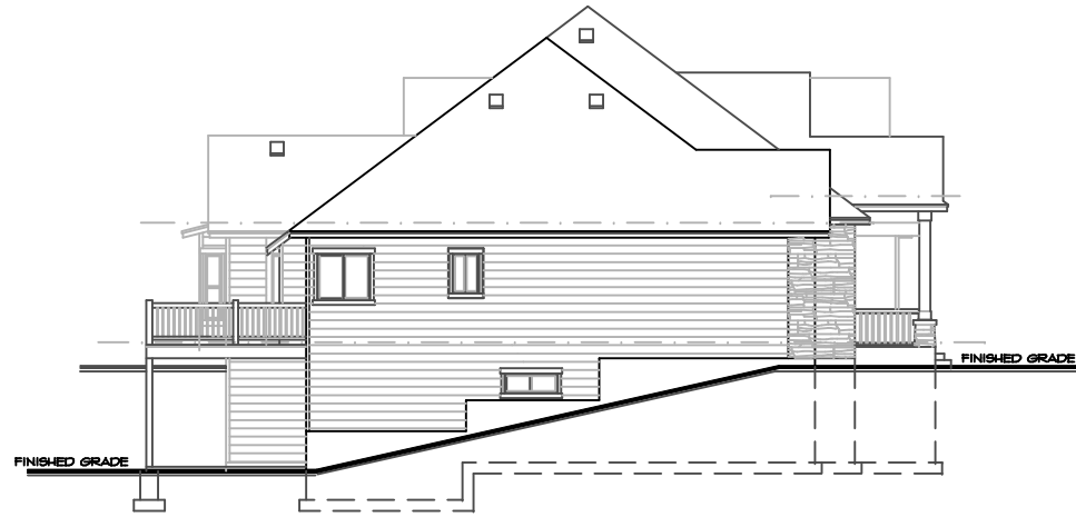
LEFT ELEVATION SCALE _____ NT6
