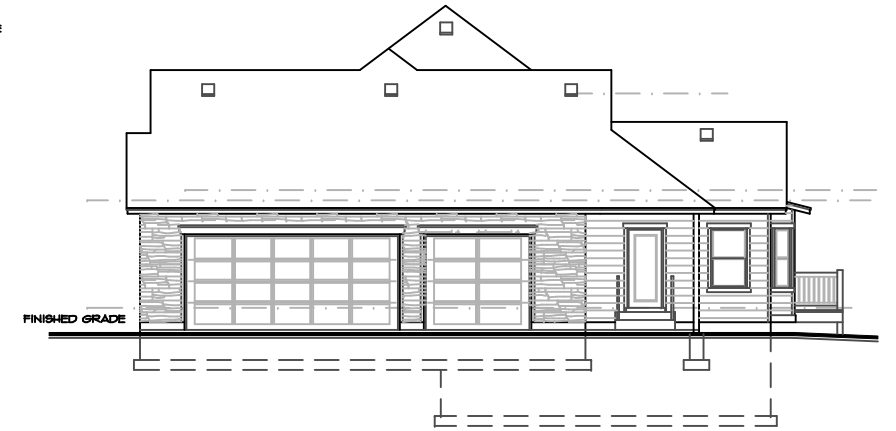
RIGHT ELEVATION SCALE _____ NT6
