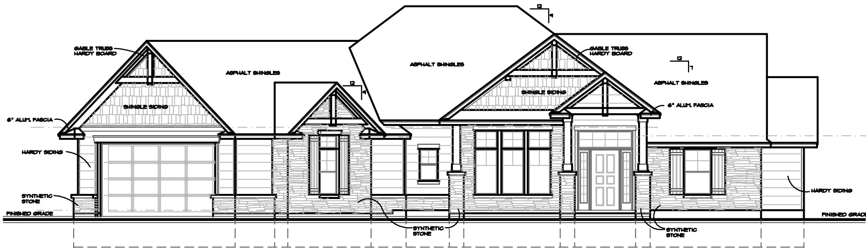
FRONT ELEVATION SCALE 1/4"
